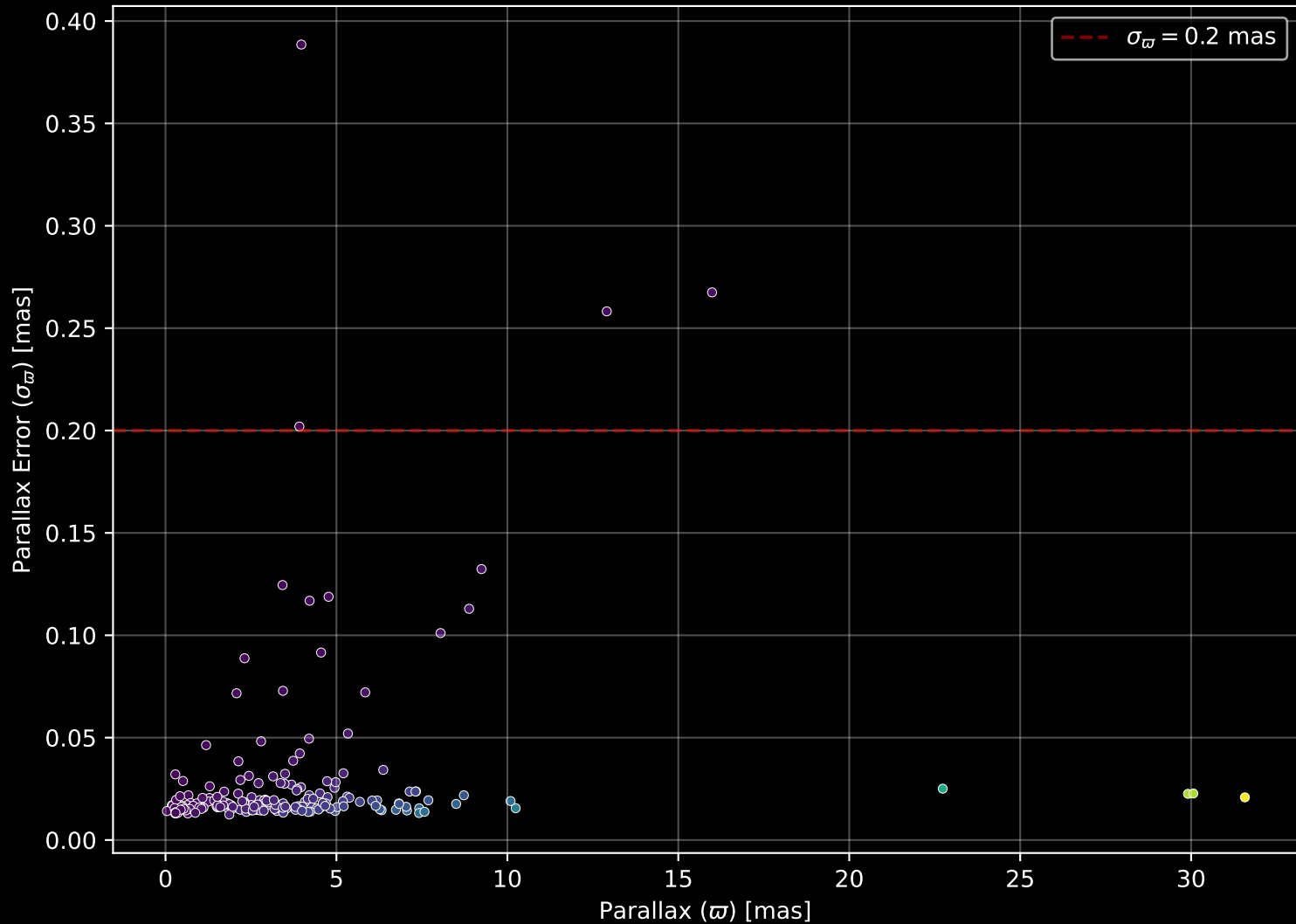
APOGEE DR17 Field: [009+52_MGA] Parallax Quality (n= 209)
