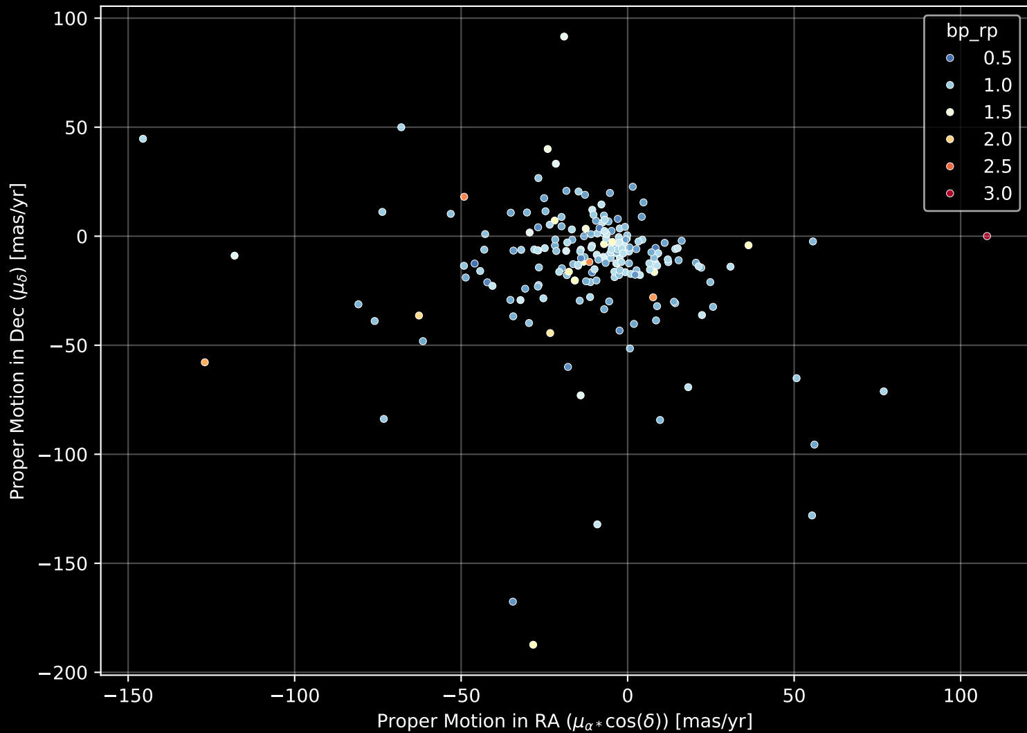
APOGEE DR17 Field: [009+52_MGA] Proper Motion Diagram (n= 209)
