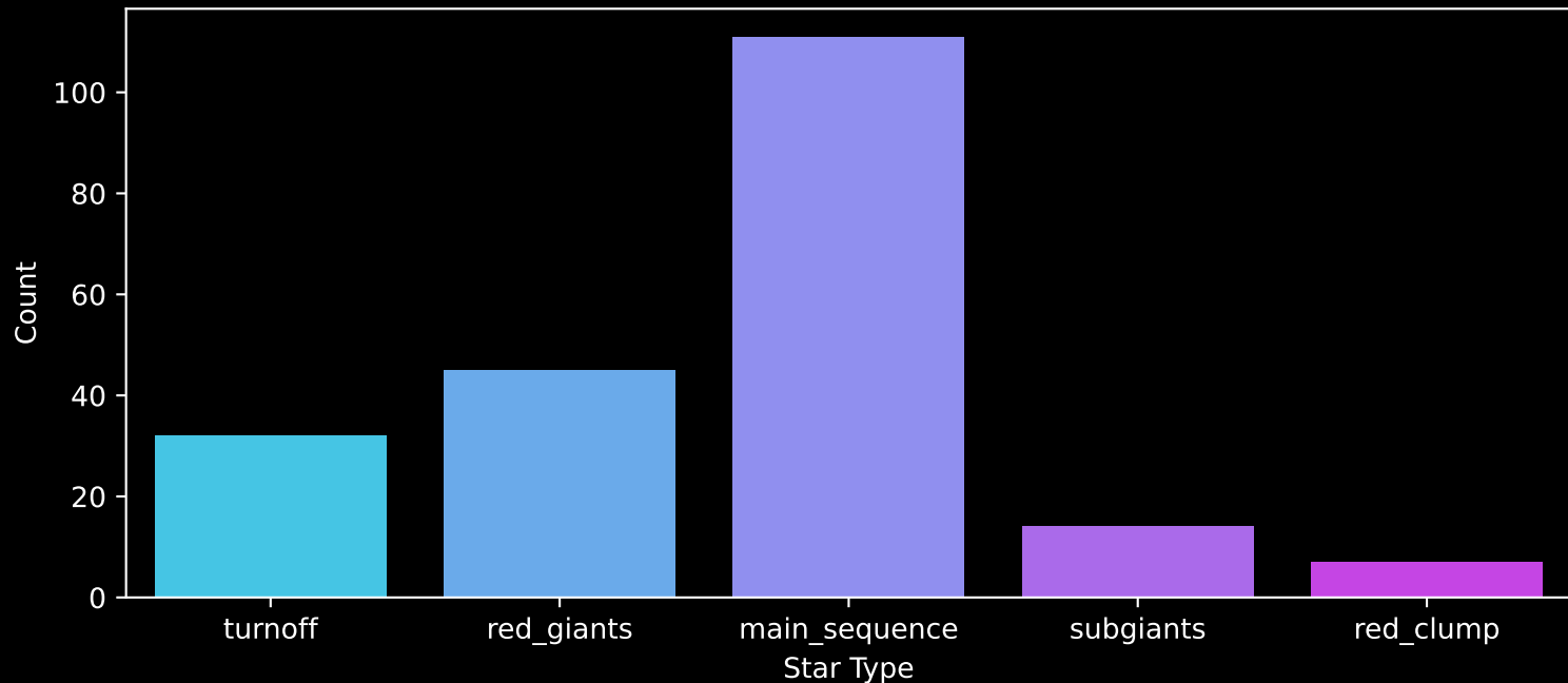
APOGEE DR17 Field: [009+52_MGA] Count plot of Star Type
