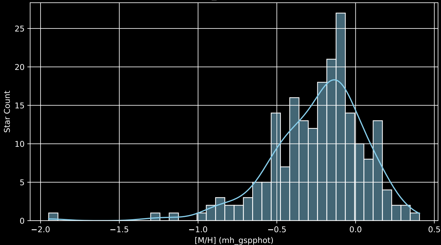
APOGEE DR17 Field: [009+52_MGA [M/H] (mh_gspphot) (n= 208)
