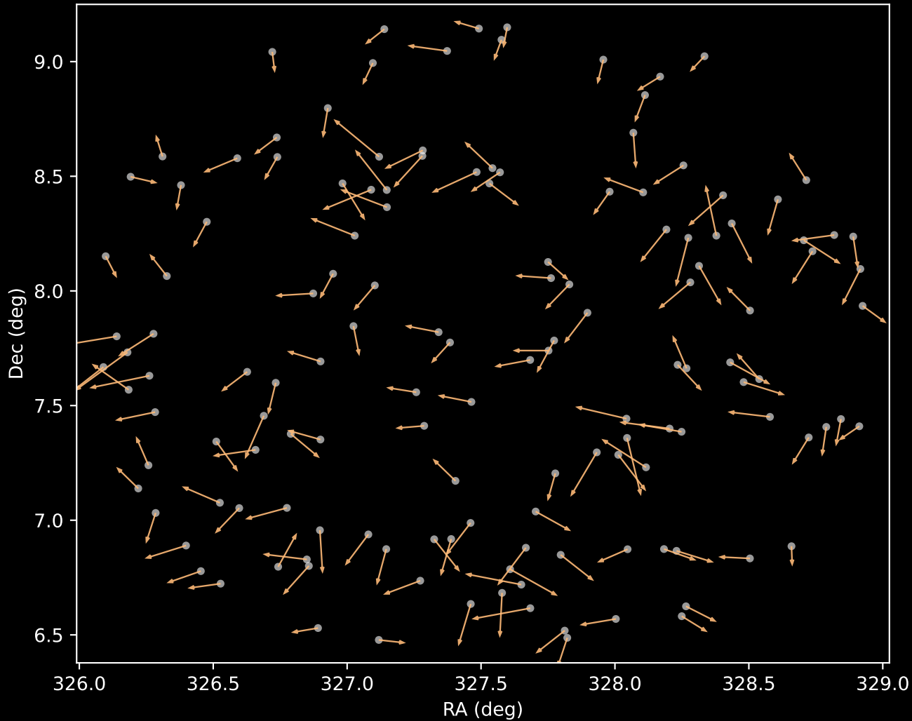
APOGEE DR17 Cluster 3 Proper Motion Vectors (n=142)
