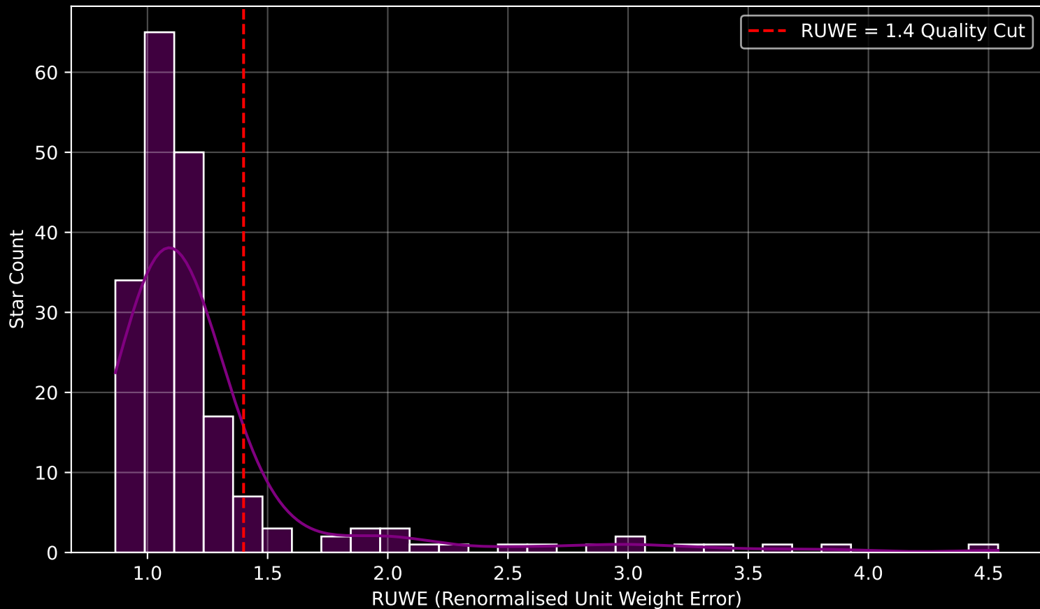
GAPOGEE DR17 Field [009+52_MGA] RUWE Distribution (n= 196)
