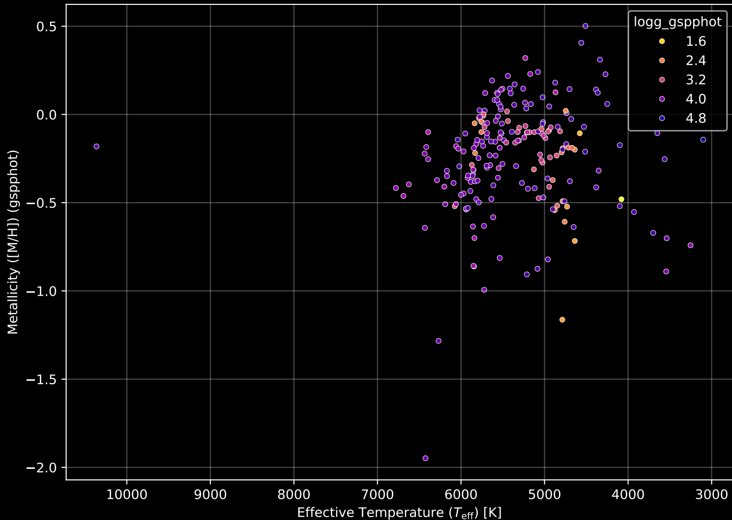
APOGEE DR17 Field: [009+52_MGA] Stellar Population Parameters (n= 209)
